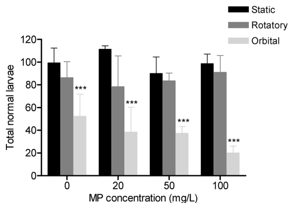
Fig. 3. Mussel larval development after exposure of embryos to PE-MP (4–6 μm) under static conditions, rotatory, and orbital shaking. Results are expressed as total normal larvae observed after 48 h. The same number of embryos was transferred into each experimental vial. Bars represent mean ± SD (n = 4). Asterisks refer to significant differences with ‘static’ treatments. *** p < 0.001.
