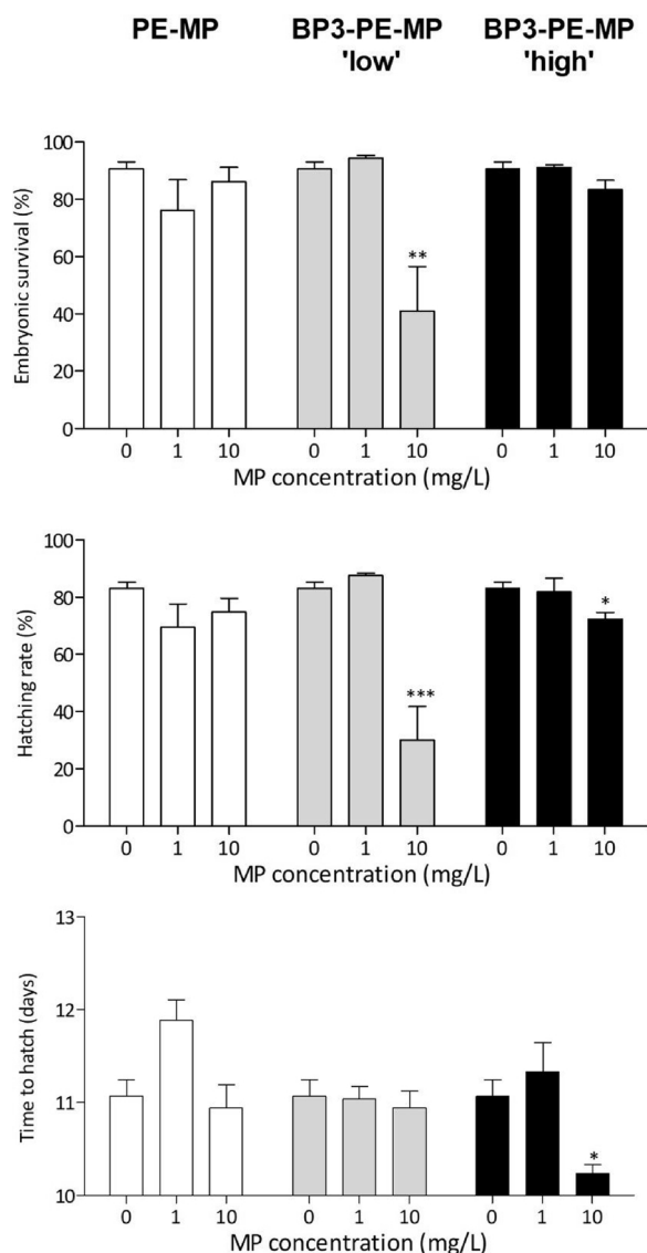
Fig. 5. Toxicity of polyethylene microplastics to Oryzias melastigma embryos. Treatments included non-spiked polyethylene microplastics (PE-MP), and PE-MP spiked with BP-3 at 'low' and 'high' concentrations (BP3-PE-MP). Embryonic survival, hatching rate, and time to hatch was recorded after 12 days of exposure. Bars represent mean \pm SD, N = 3-6 . Asterisks refer to significant differences to the control treatment (C). * p < 0.05 , ** p < 0.01 , *** p < 0.001 .
