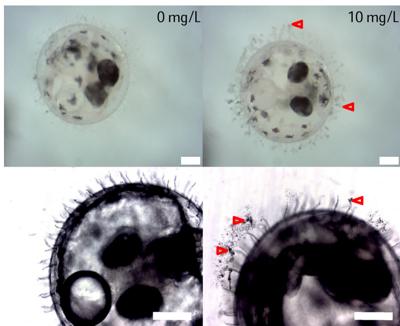
Fig. 2. Oryzias melastigma embryos exposed to 0 and 10 mg PE-MP L -1 (4–6 μm). Embryos are in direct contact with microplastics stuck on villi at the surface of the chorion. White scale bars 200 μm.
