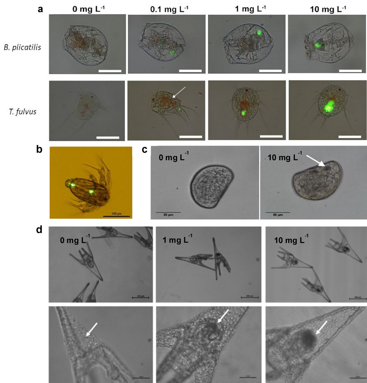
Fig. 1. Ingestion of microplastics. a , B. plicatilis and T. fulvus nauplii revealing fluorescent polyethylene microparticles (PE-MP) inside. Note that copepods did not ingest PE-MP at 0.1 mg L -1 (arrow). Scale bars are 100 \mu m. b , A. clausi nauplius larvae with fluorescent PE-MP accumulated on the gut. Scale bar 100 \mu m. c , M. galloprovincialis larvae revealing PE-MP inside. Scale bar 50 \mu m. d , P. lividus larvae, notice the transparent stomachs in 0 mg L -1 in contrast with the dark filled stomachs in the other treatments. Top images \times 10 magnification, scale bars 200 \mu m and down images \times 40 magnification, scale bars are 50 \mu m.
