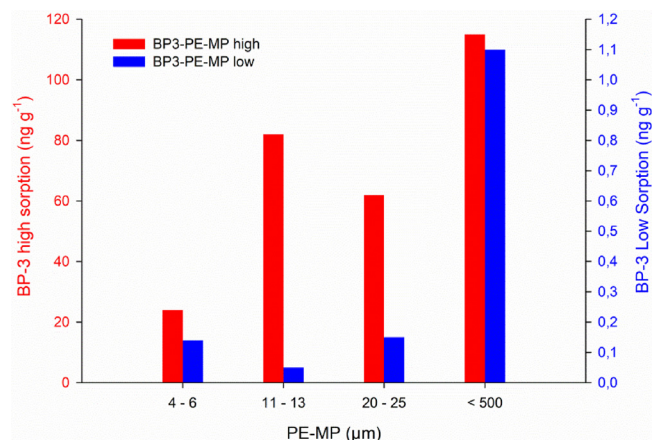
Fig. 4. BP-3 sorption on the different polyethylene microparticles (PE-MP) incubated at low and high BP-3 concentrations.
